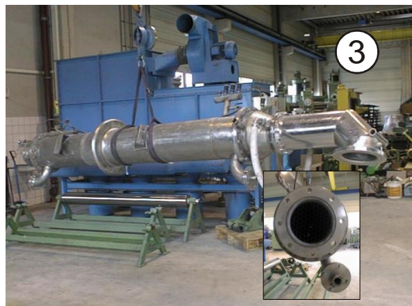
heat-exchanger, cyclone - filter/separation
