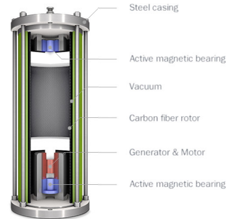
Fly wheel, source: Stornetic GmbH Sintered magnets, source: BEC GmbH
